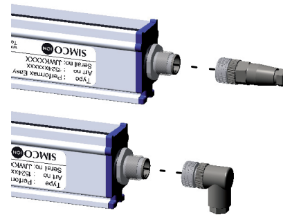
Separate connector, straight or angled
