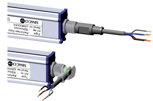
Straight connector with cable
