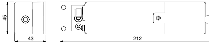
Technical drawing CM Tiny
